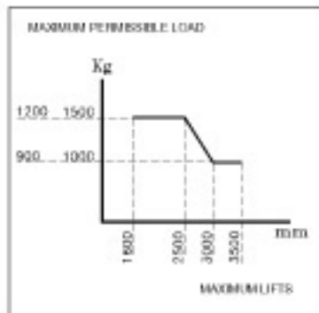
Diagram of maximum loads regarding the lifts.
