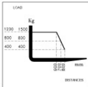
Diagram representing the position variation of the load barycenter with the variation of the same.
